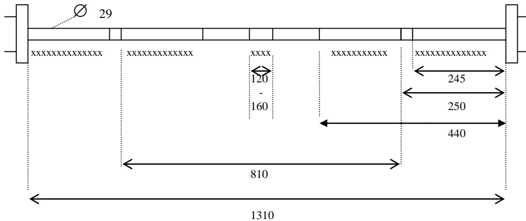
Measurements in mm (knurling distances inside the collar sleeves)
